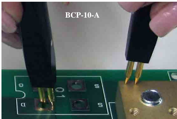
Pin spacing: 0.156" on center Probe tip removable Shown Here BCP-10-C
